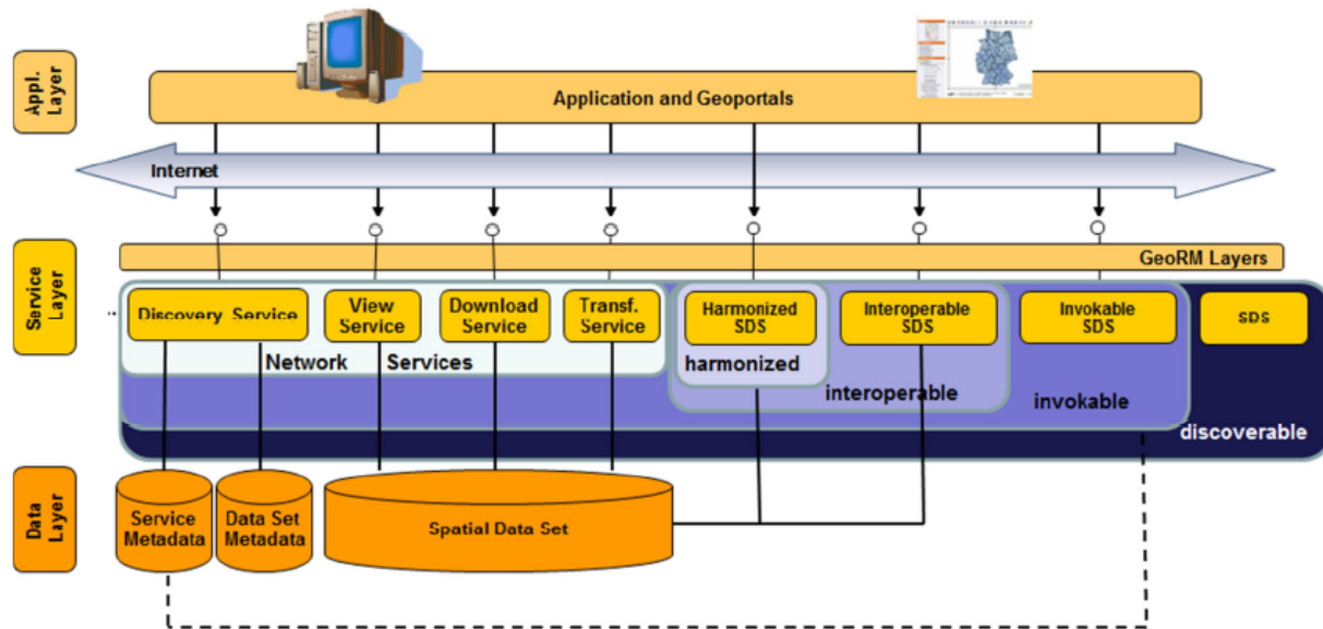
Figure 1 Updated INSPIRE Architecture
